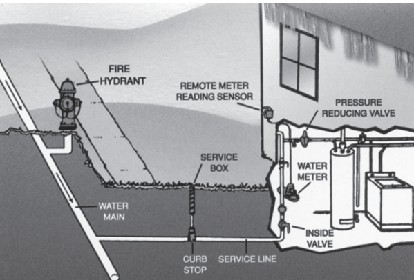
Typical water system set-up
